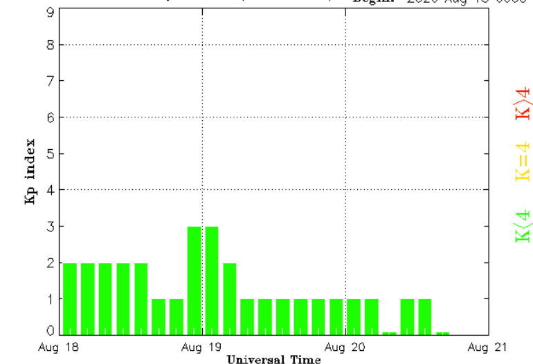
Estimated Planetary K index (3 hour data) Begin: 2020 Aug 18 0000 UTC
