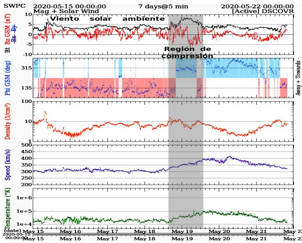
Imagen 3: http://www.swpc.noaa.gov/products/real-time-solar-wind
