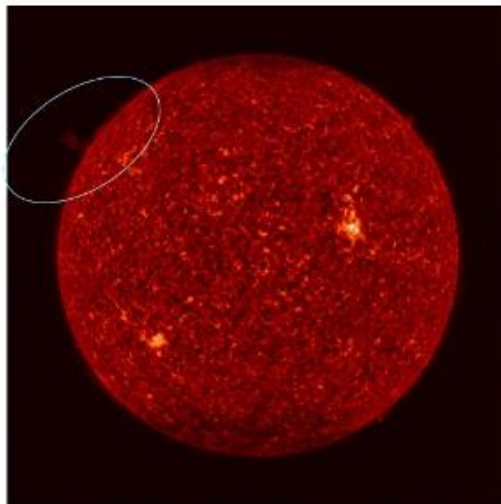
SDO AIA 304 A
