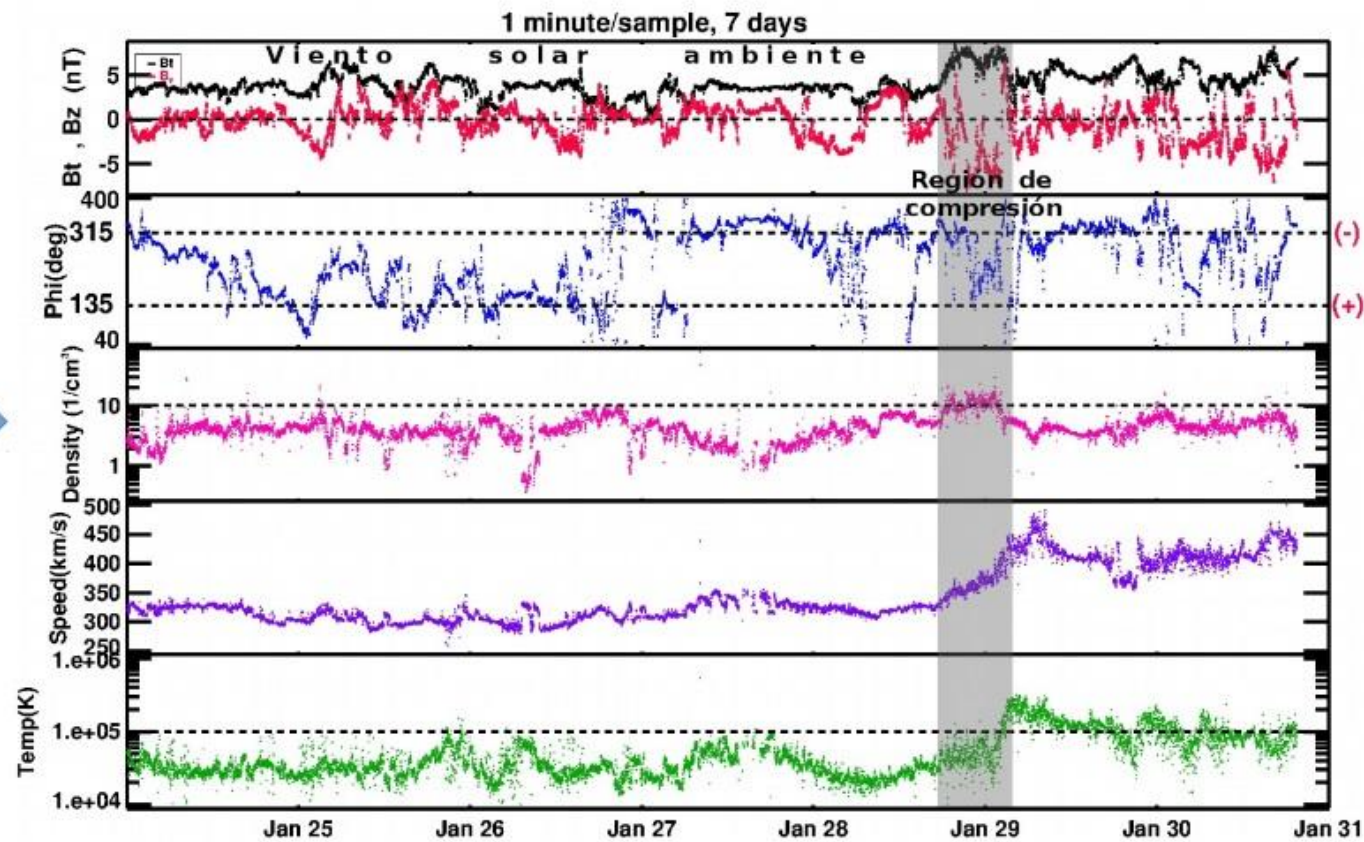
Imagen 2: http://www.swpc.noaa.gov/products/real-time-solar-wind
